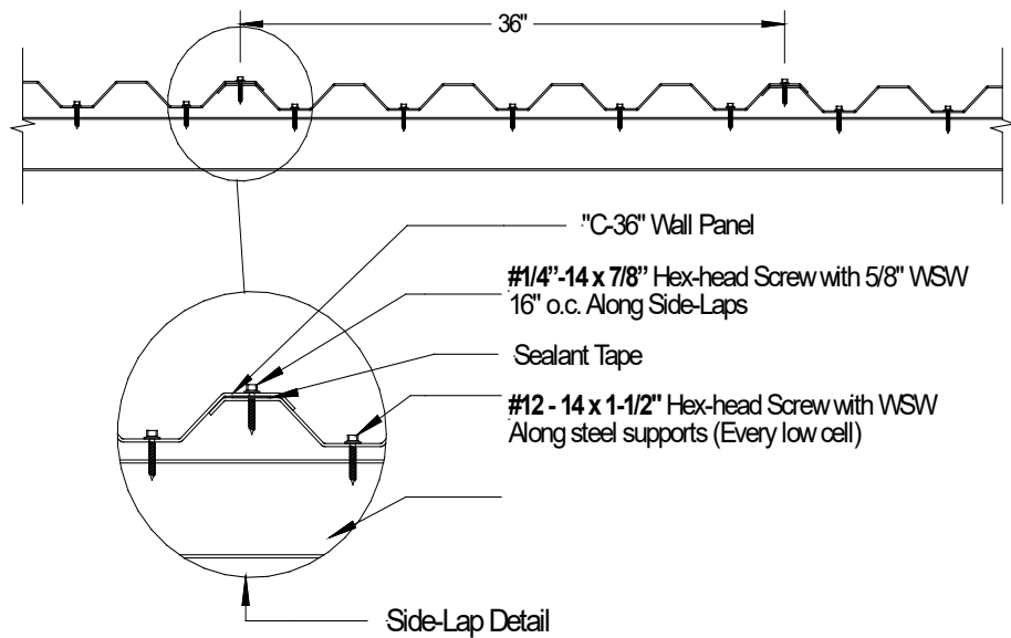
TYPICAL ASSEMBLY PROFILE VIEW (TYPICAL FASTENING PATTERN ALONG SUPPORTS)
