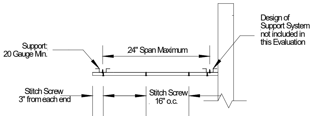
TYPICAL ASSEMBLY SECTION VIEW
